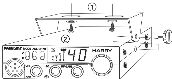
MOUNTING DIAGRAM
